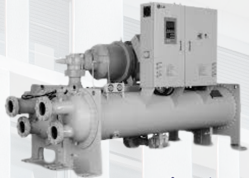
LG Water-cooled Screw Chiller is equipped with a highly efficient load evaporator and oil recovery system for reliable operation.
